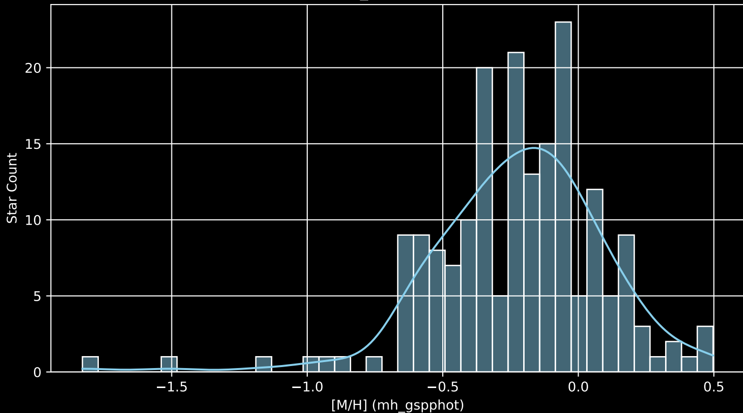
APOGEE DR17 Field: [073+53_MGA [M/H] (mh_gspphot) (n= 188)
