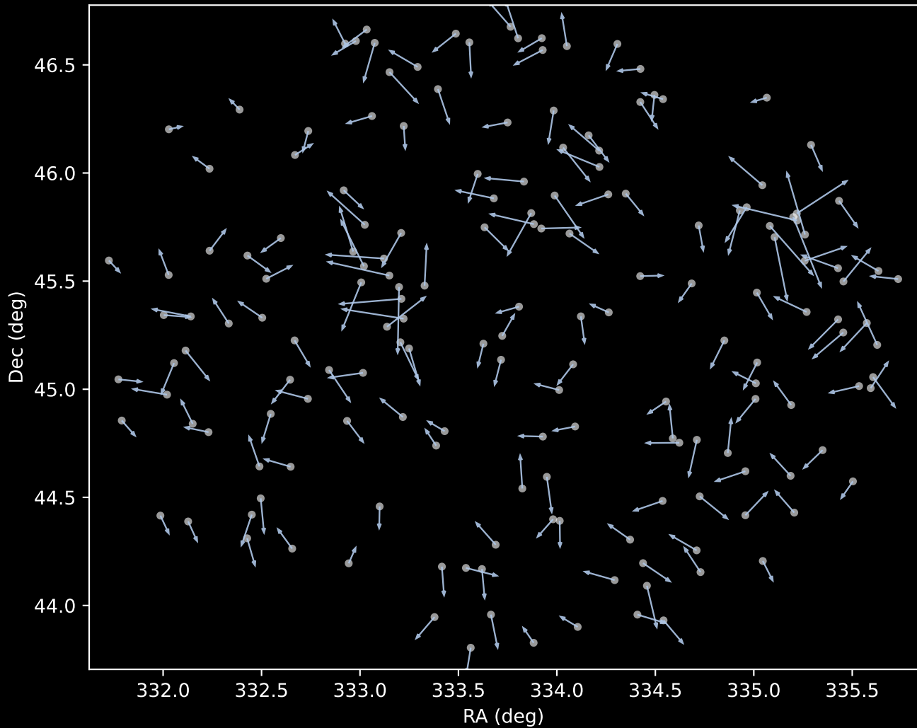
APOGEE DR17 Cluster 1 Proper Motion Vectors (n=174)
