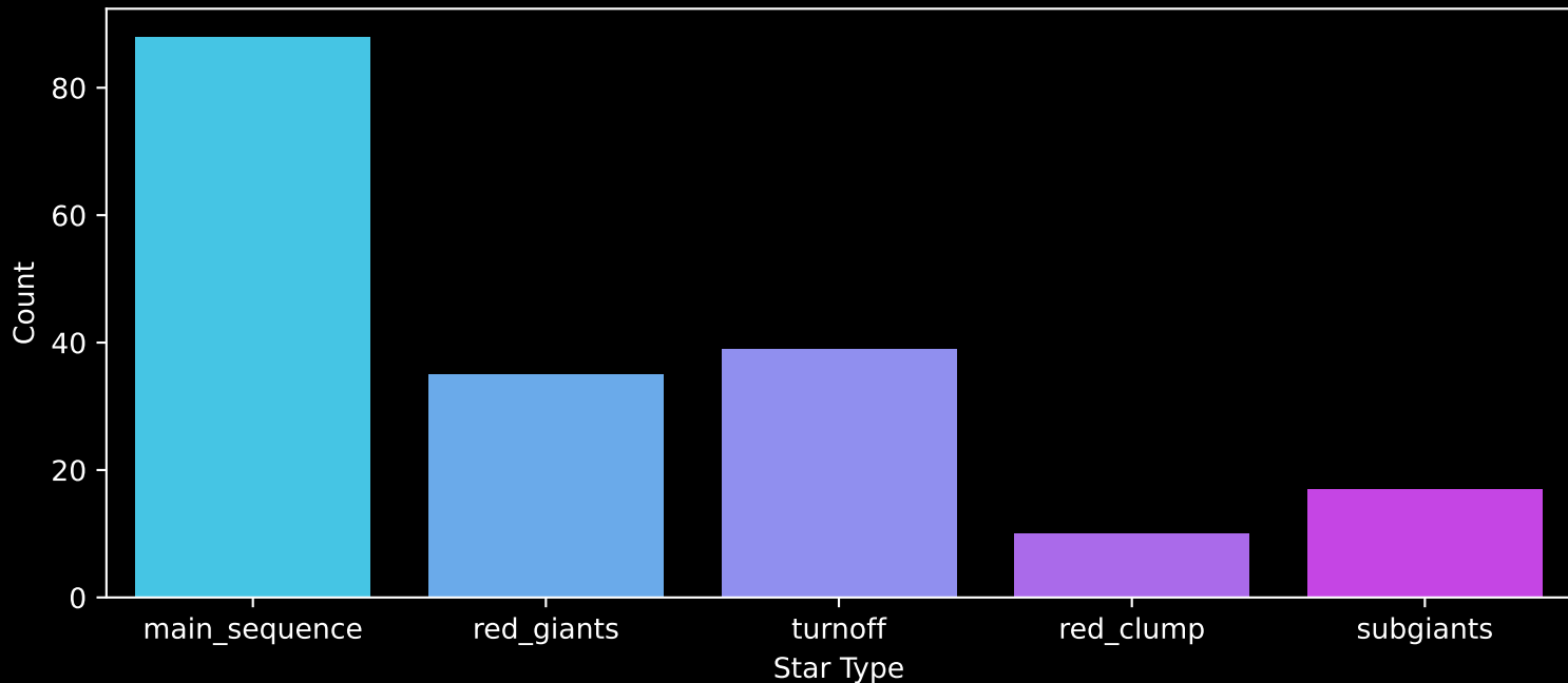
APOGEE DR17 Field: [073+53_MGA] Count plot of Star Type
