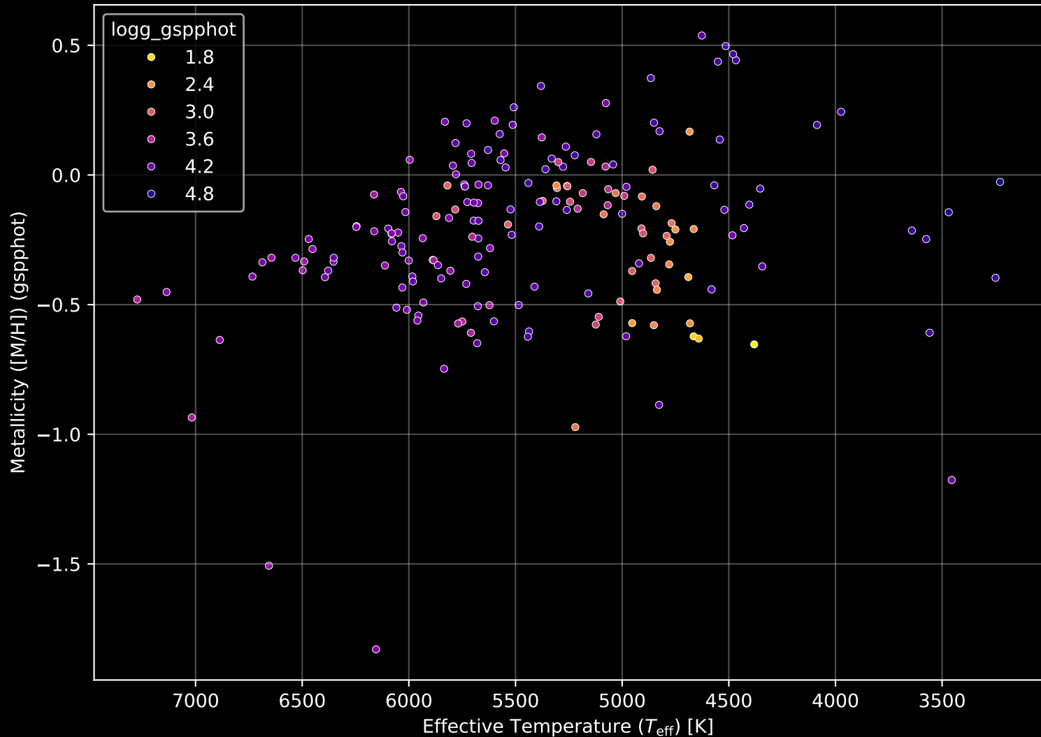
APOGEE DR17 Field: [073+53_MGA] Stellar Population Parameters (n= 189)
