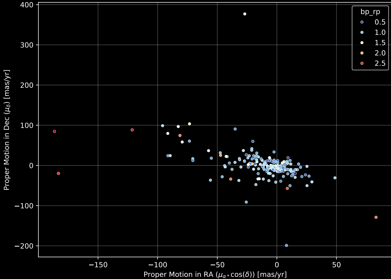
APOGEE DR17 Field: [073+53_MGA] Proper Motion Diagram (n= 189)
