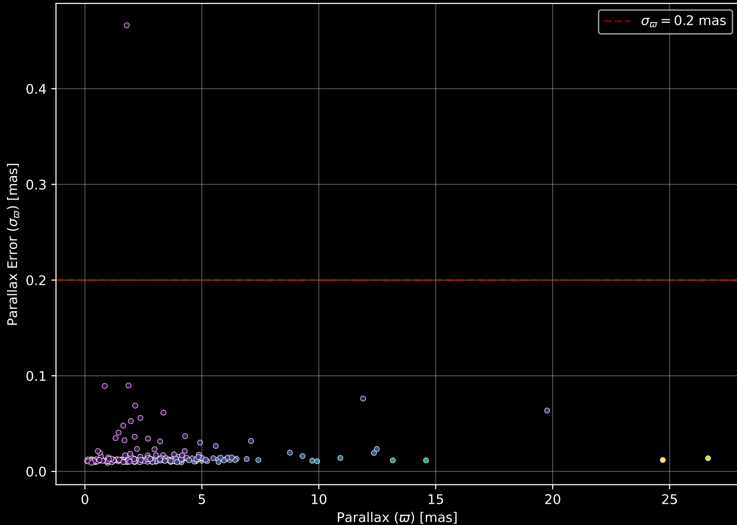
APOGEE DR17 Field: [073+53_MGA] Parallax Quality (n= 189)
