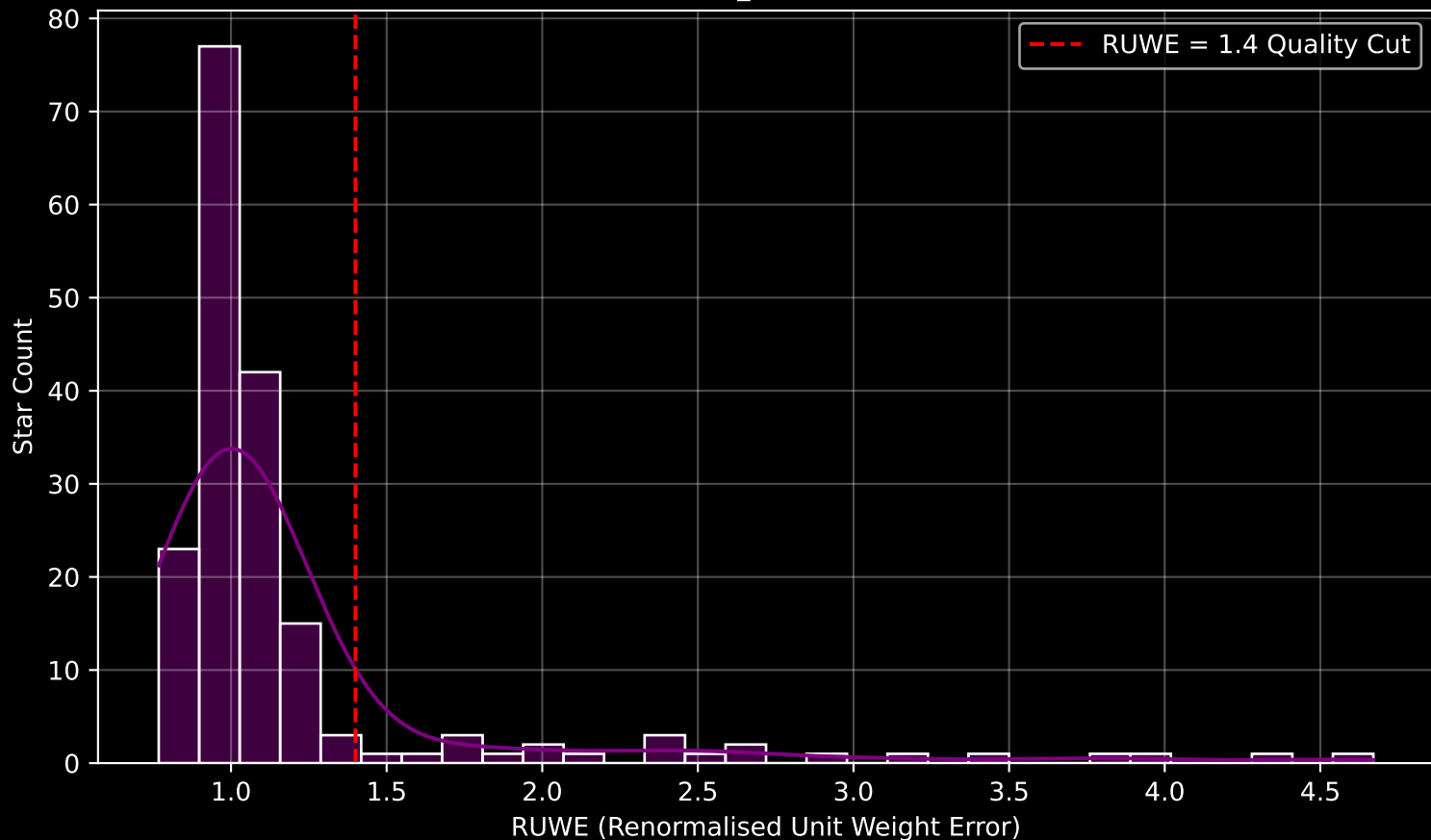
GAPOGEE DR17 Field [073+53_MGA] RUWE Distribution (n= 182)
